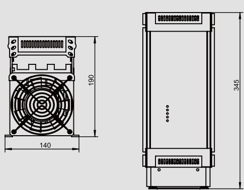
GSM3E40250D 长宽高:345mm*140mm*190mm
